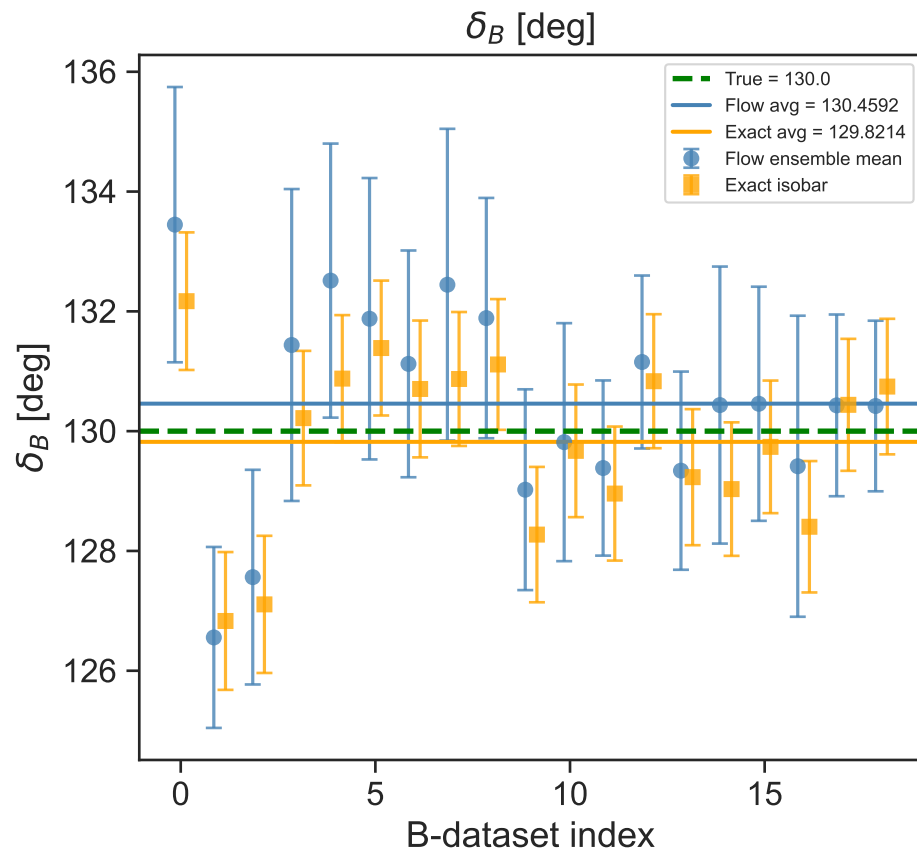
Fitted values across 19 B-datasets
